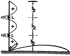
Franklin loaded vertical antenna, showing vertical radiation pattern for all directions (solid curves) and current distribution curves (dotted).
